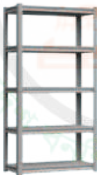
STEEL RACK BFIDC-3 (PROVIDER) MODEL NO: BSOR 25003 Size: 1150 x 460 x 1830 mm Material: Mild Steel (MS). Paint: Powder Coated Finish.
