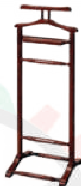
WOODEN CLOTH STAND BFIDC-6 MODEL NO: BWCS 25006 Size: Size: 450 x 28,50 x 1250 mm Material: Solid Wood. Polish: Natural/Lacquer.
