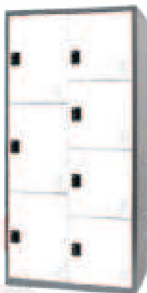
STEEL PERSONAL LOCKER BFDC-5 (PROVIDER) MODEL NO: BSPL 25005 Size: 915 x 400 x 1830 mm Material: Mild Steel (MS). Paint : Powder Coated Finish.
